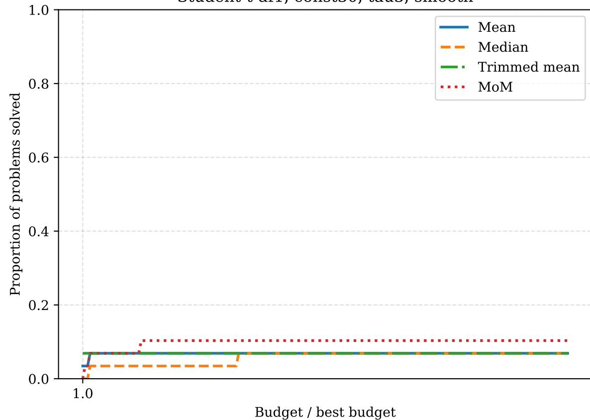
Student-t df1, const30, tau3, smooth
