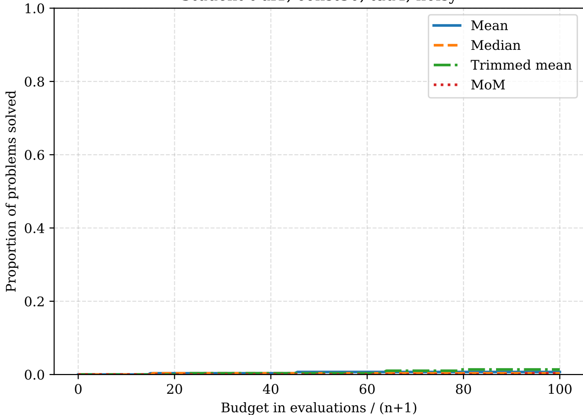
Student-t df1, const30, tau4, noisy
