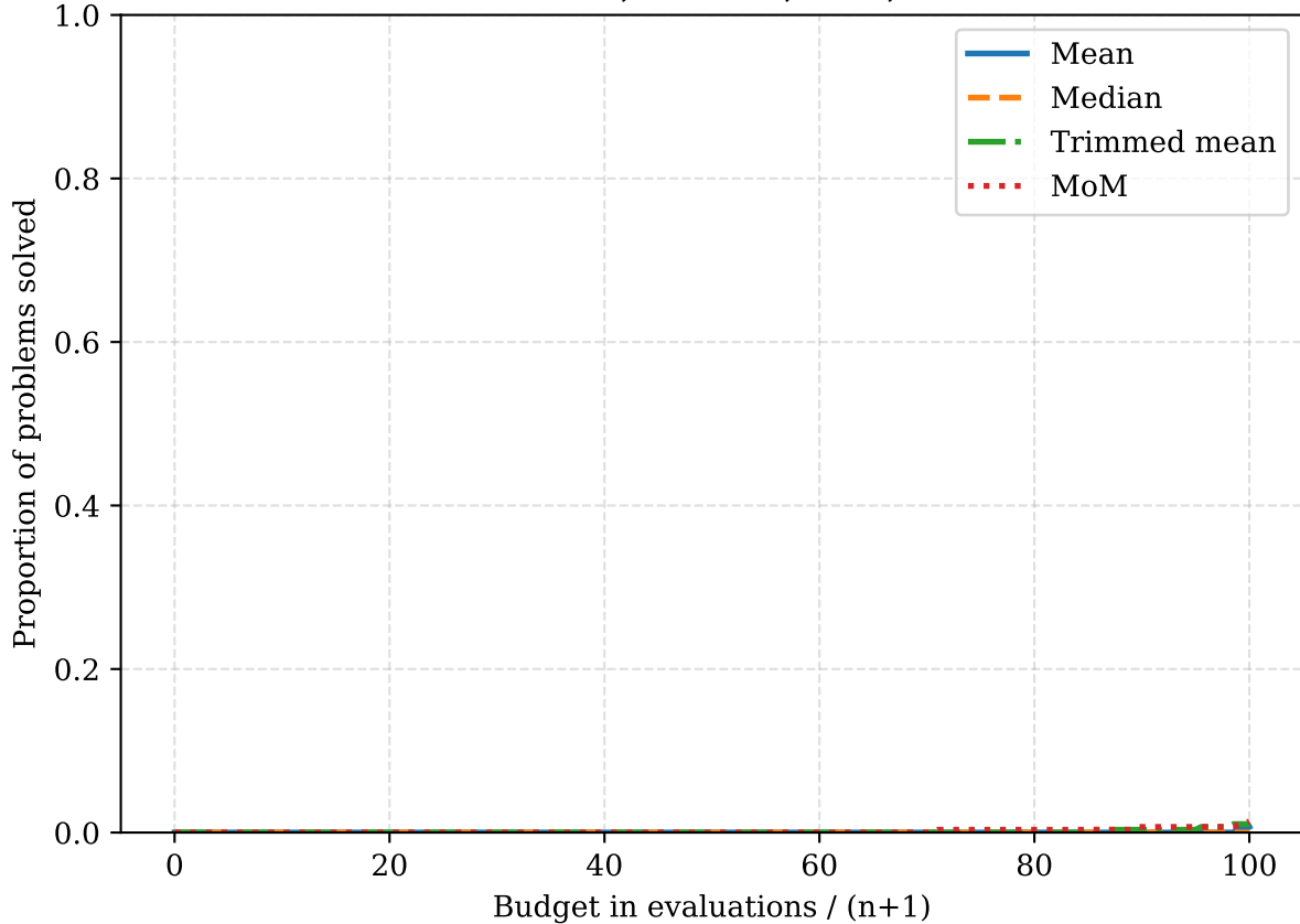
Student-t df1, const30, tau5, smooth
