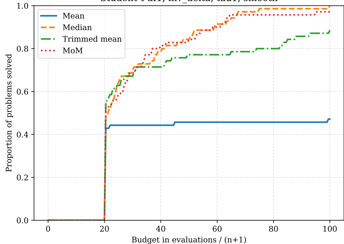
Student-t df1, inv_delta, tau1, smooth
