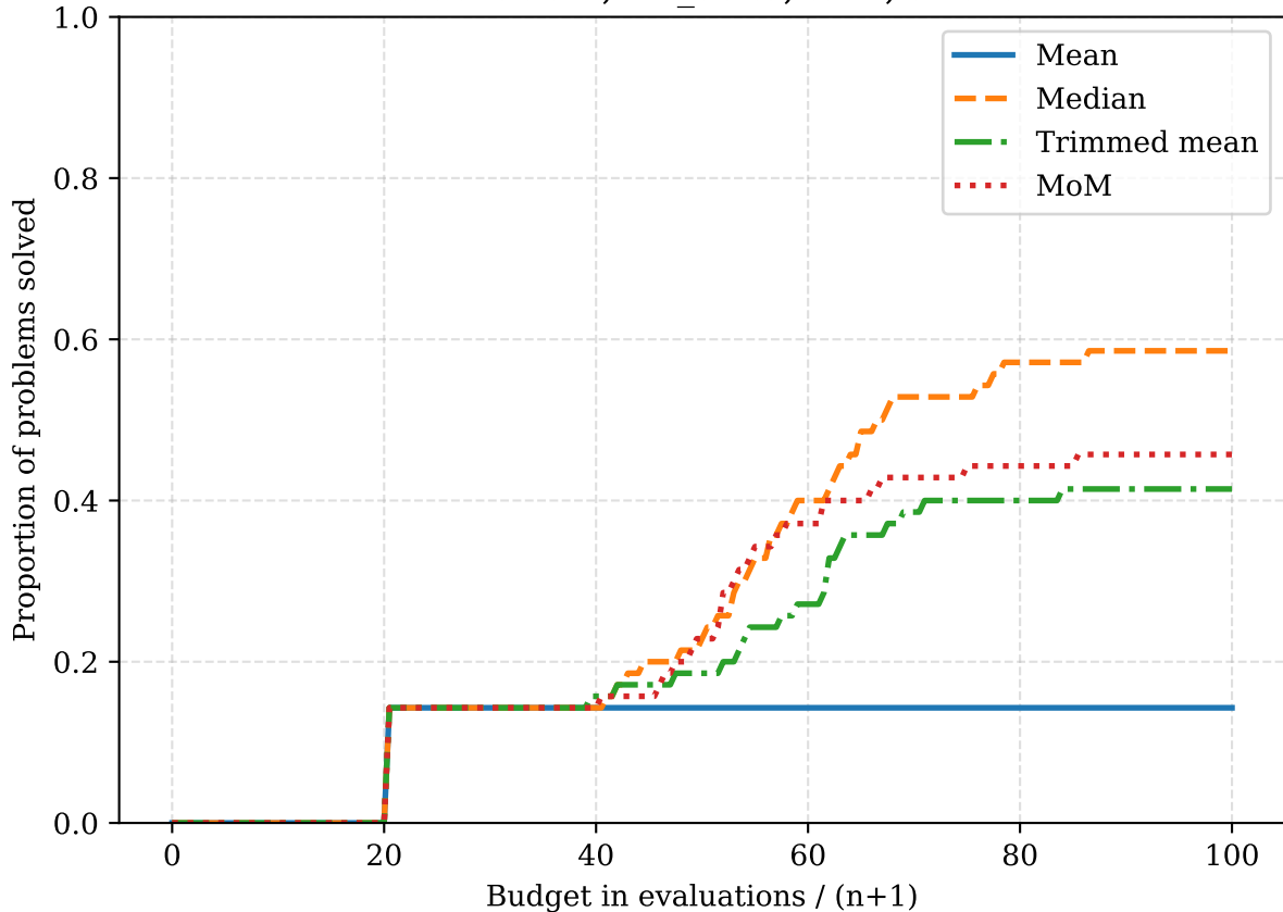
Student-t df1, inv_delta, tau2, smooth
