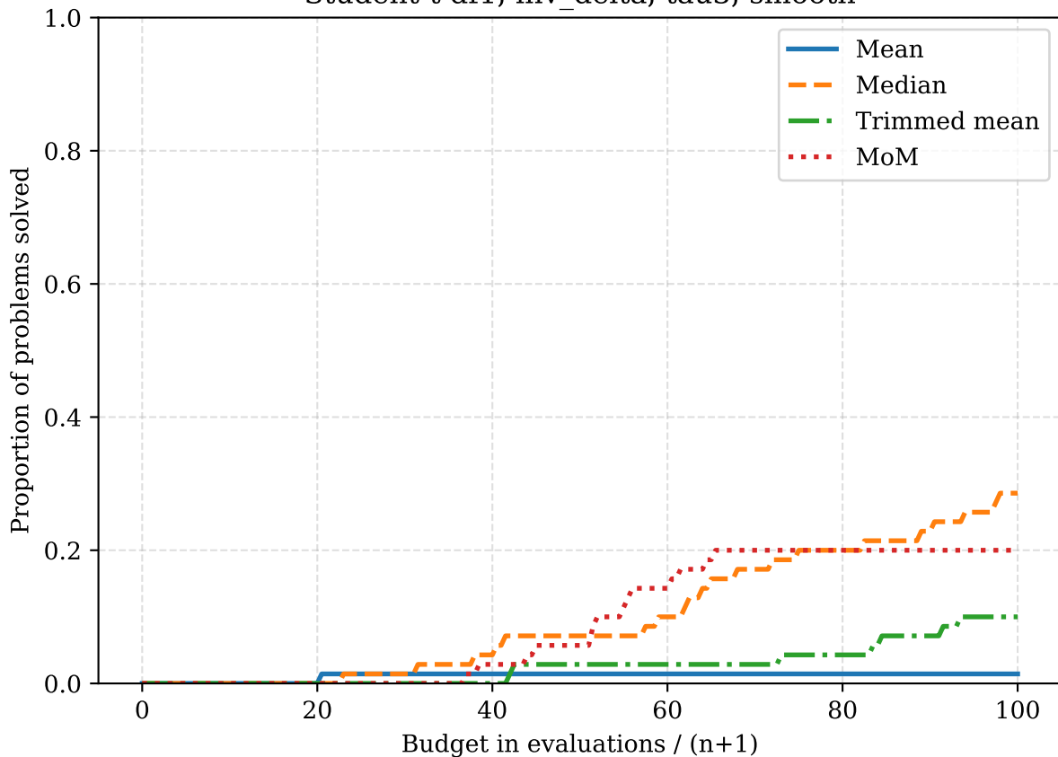
Student-t df1, inv_delta, tau3, smooth
