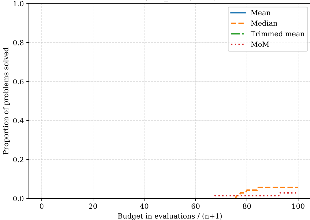
Student-t df1, inv_delta, tau4, smooth
