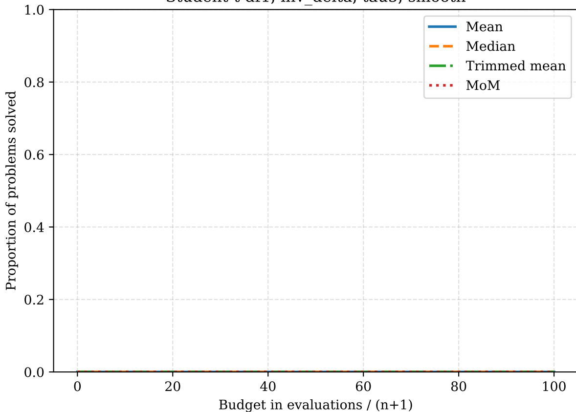
Student-t df1, inv_delta, tau5, smooth
