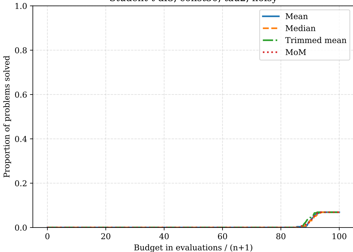
Student-t df3, const30, tau2, noisy
