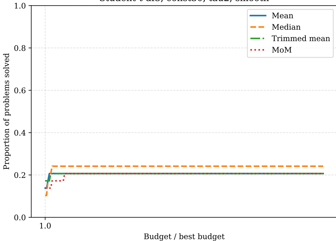
Student-t df3, const30, tau2, smooth
