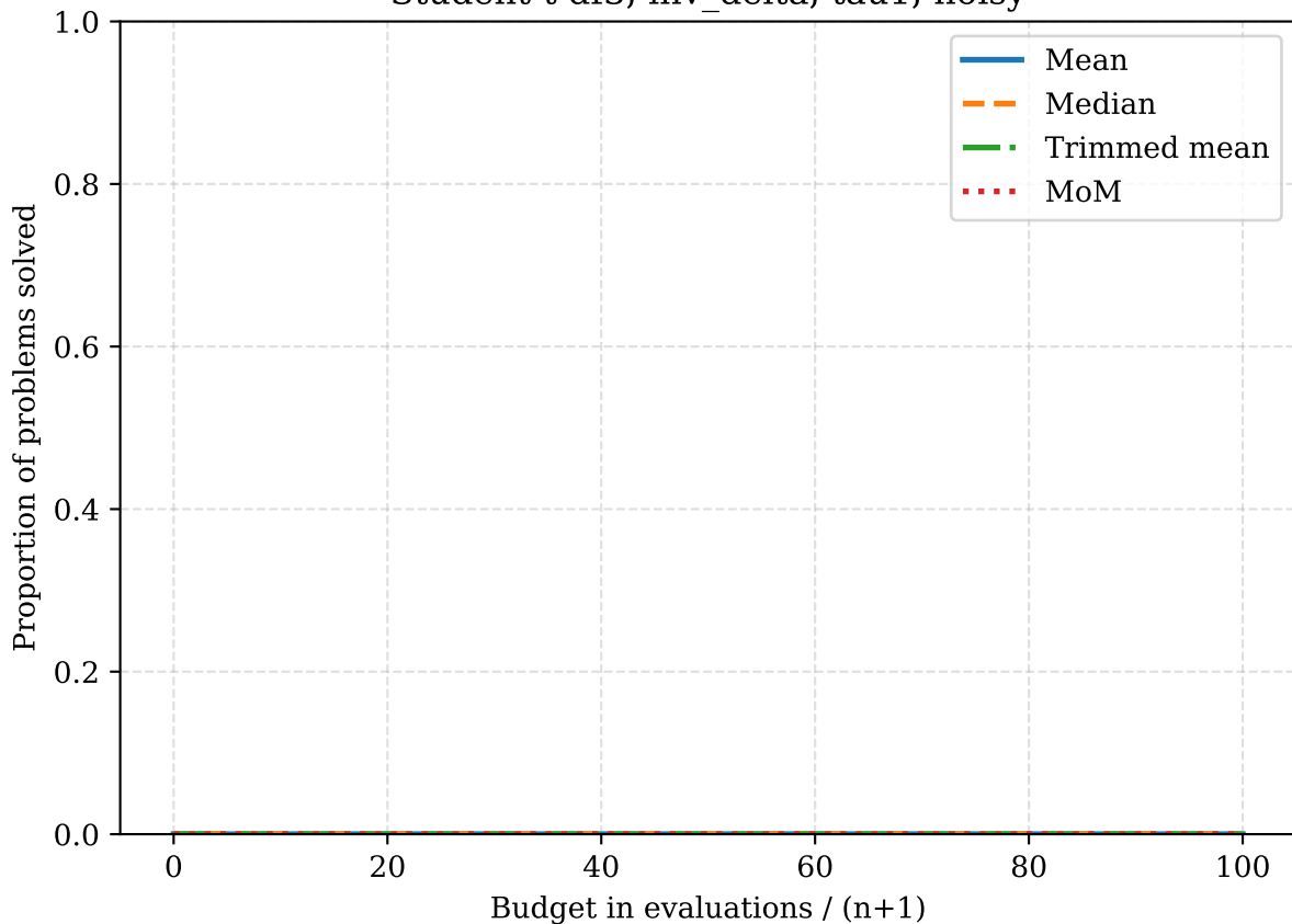
Student-t df3, inv_delta, tau1, noisy
