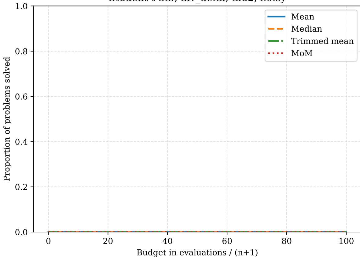
Student-t df3, inv_delta, tau2, noisy
