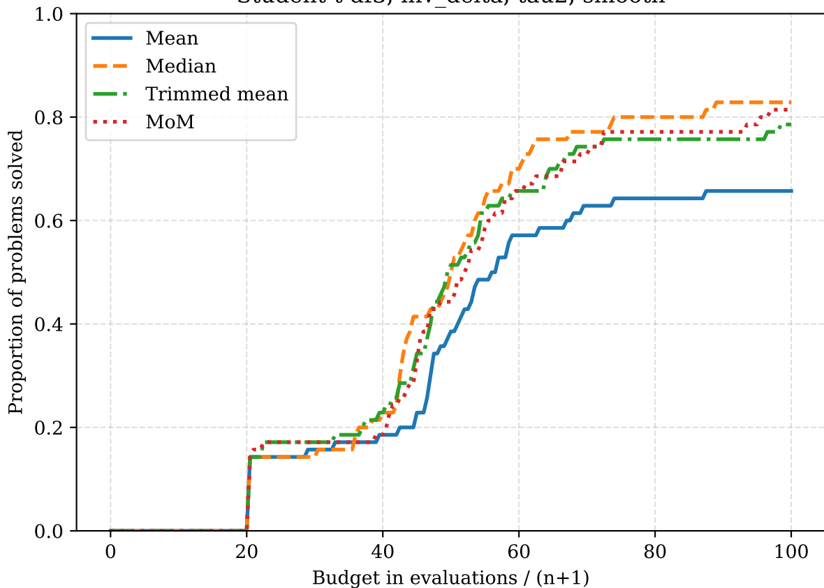
Student-t df3, inv_delta, tau2, smooth
