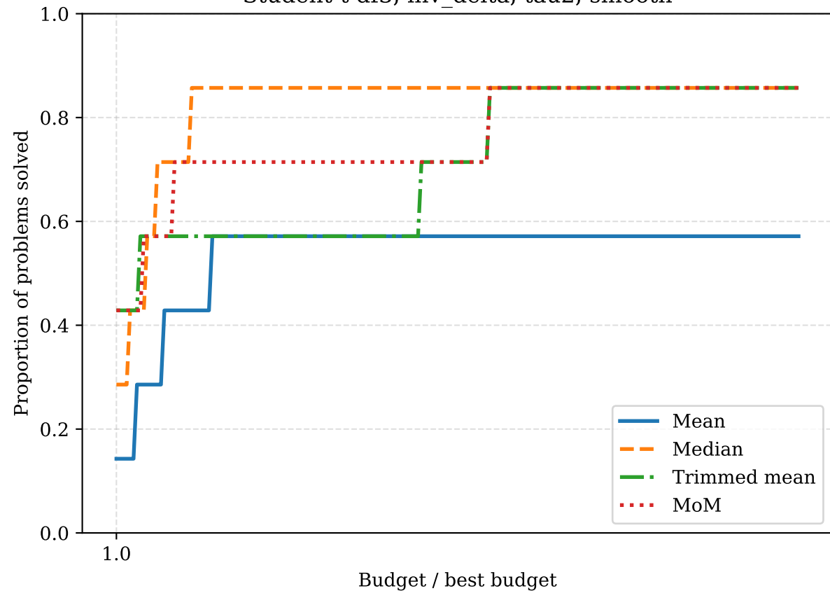
Student-t df3, inv_delta, tau2, smooth
