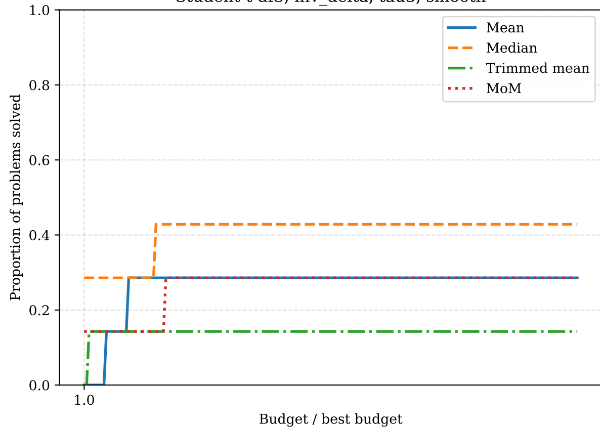
Student-t df3, inv_delta, tau3, smooth
