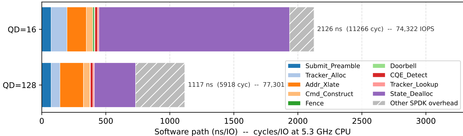
Per-IO software cost decomposition (4096B random read, SPDK)
