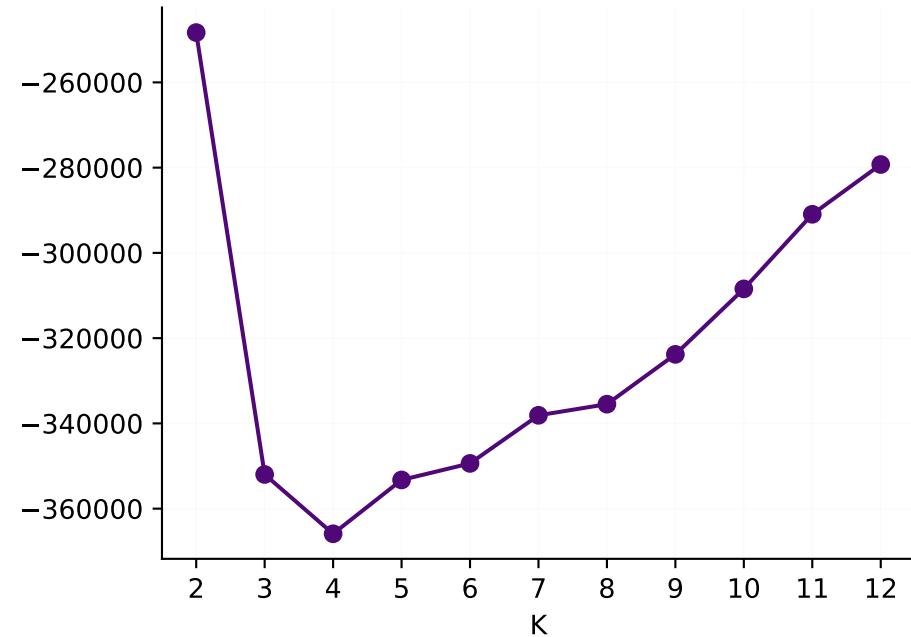
BIC (lower=better)
