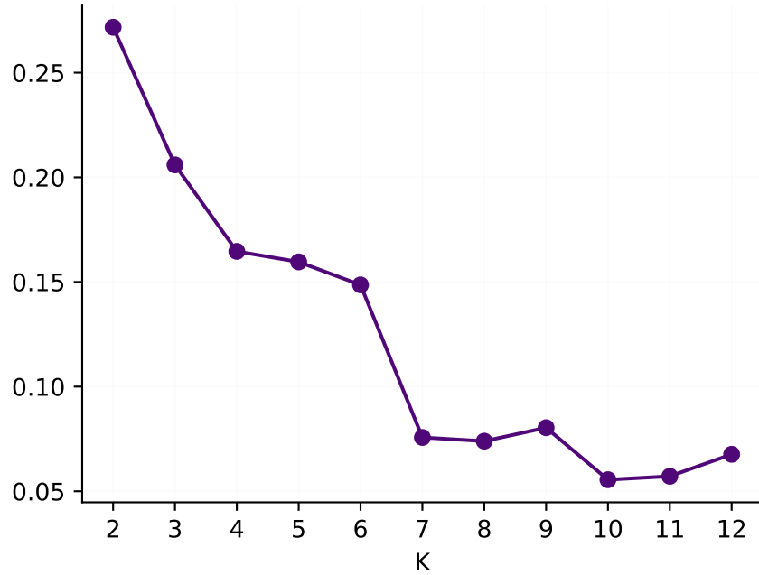
BIC (lower=better)
