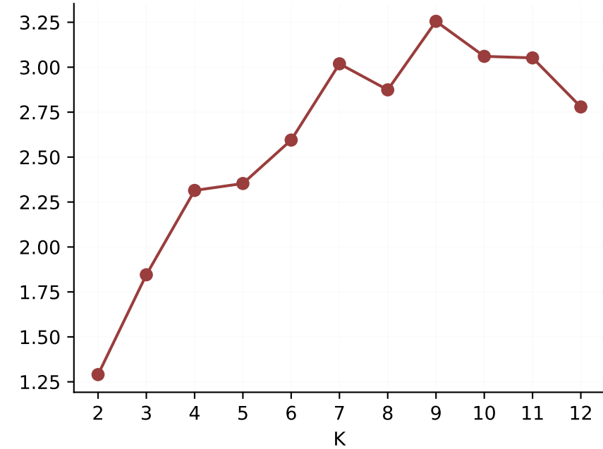
Davies-Bouldin (lower=better)
