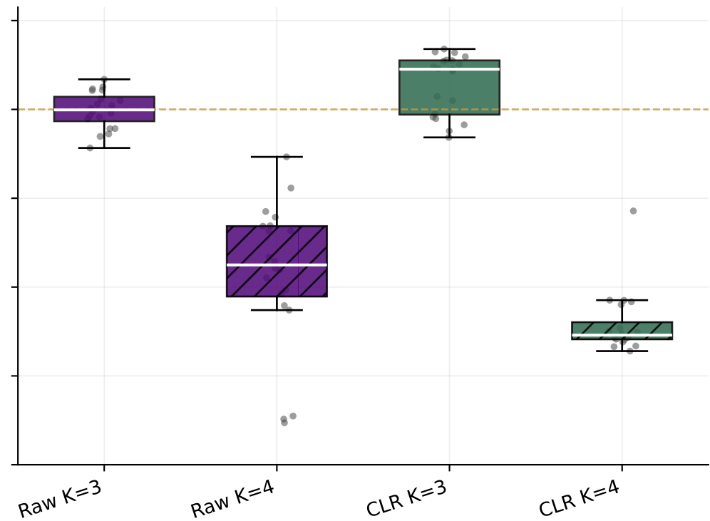
Weakest matched cluster (Jaccard)
