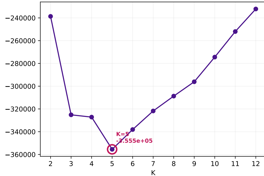
BIC (lower=better)
