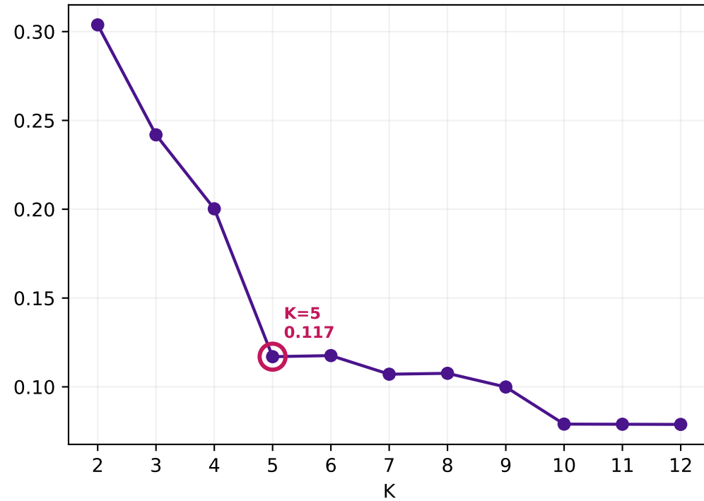
BIC (lower=better)
