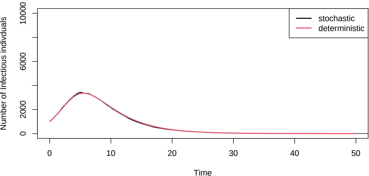
Stochastic vs. Deterministic when size of population = 10000
