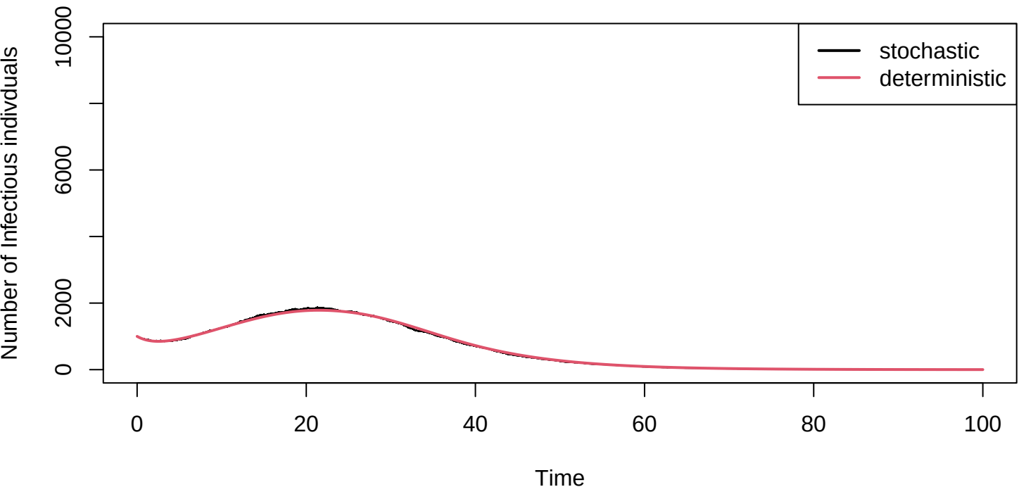
stochastic vs deterministic for SEIR model with \beta(t) when N = 10000
