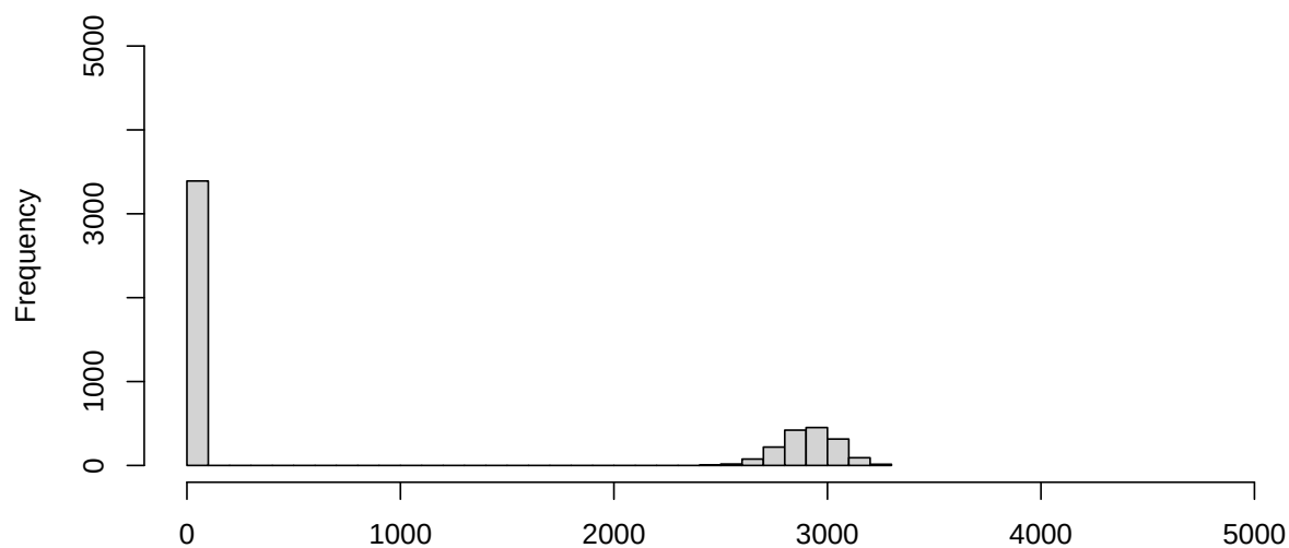
Histogram of final size when N=5000
