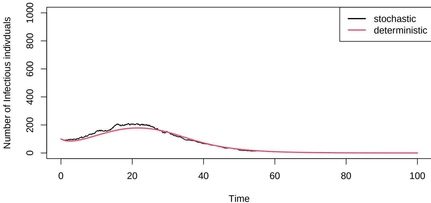
stochastic vs deterministic for SEIR model with \beta(t) when N = 1000
