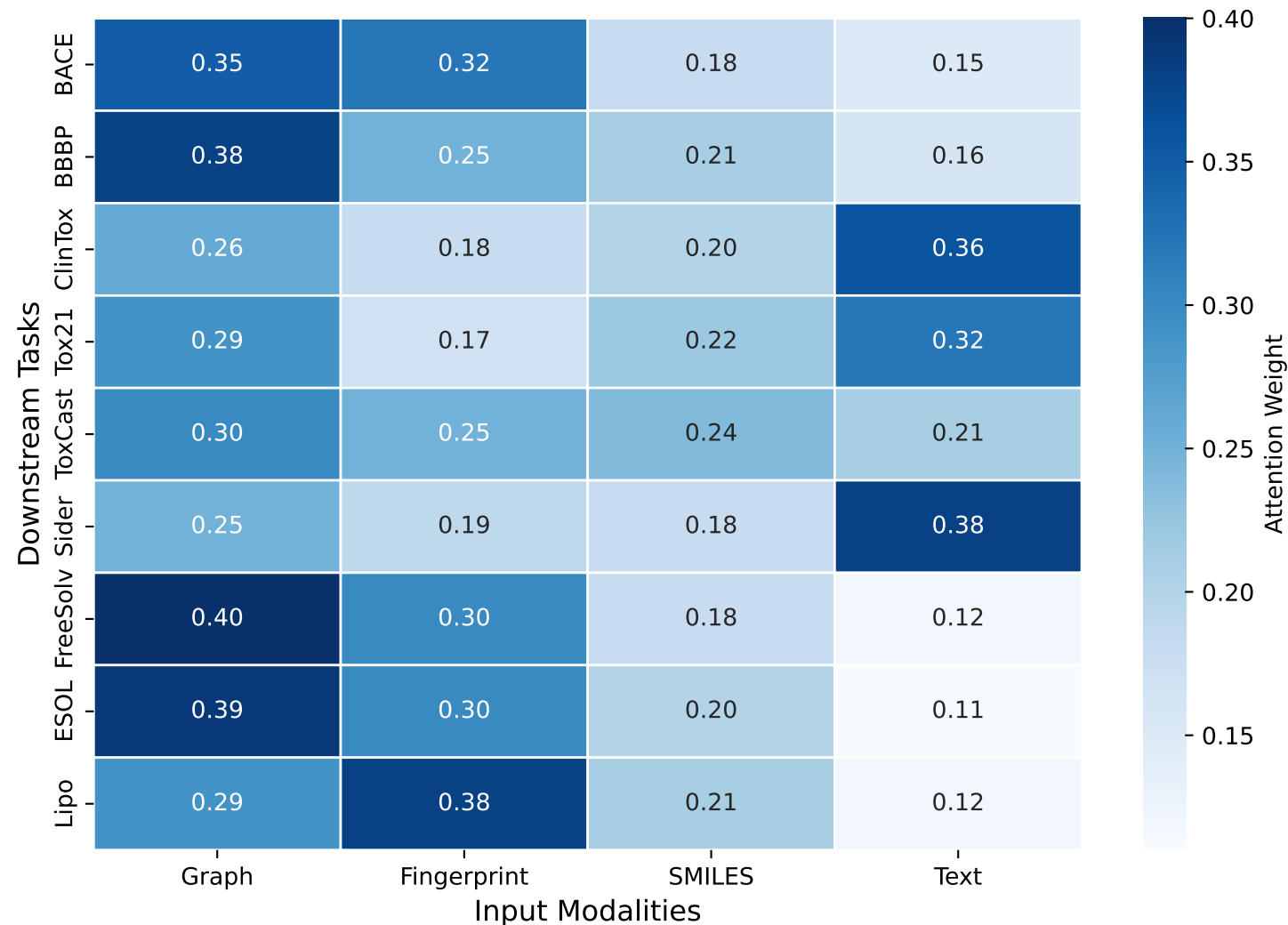
Multi-modal Attention Weights across Molecular Tasks
