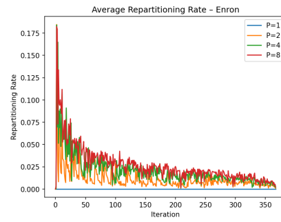
Figure 11: Enron
