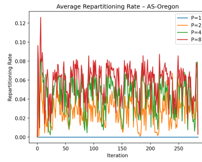
Figure 10: AS-Oregon
