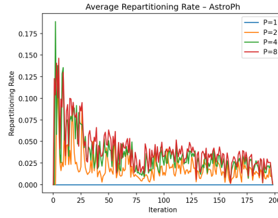
Figure 9: AstroPh
