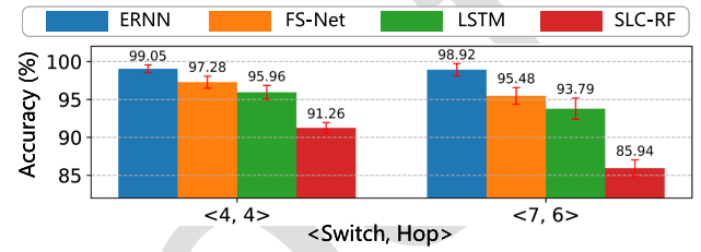
Fig. 9. Model accuracy in serial network structure.
