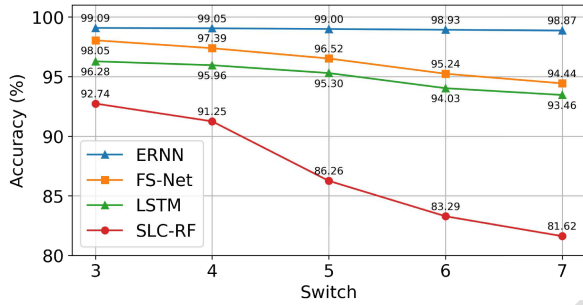
Fig. 7. Model accuracy in parallel network structure.
