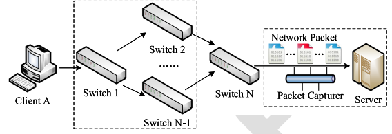
Fig. 6. Network topology with parallel structure.
