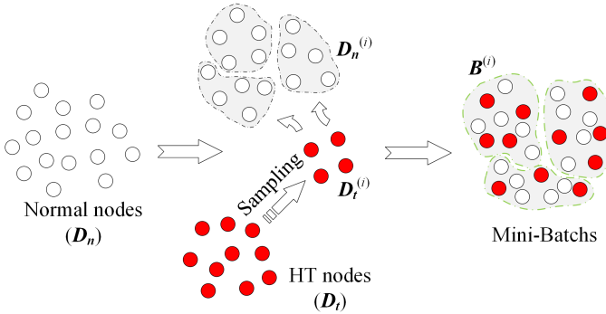
Fig. 5. Imbalanced dataset handling.
