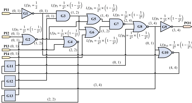
Fig. 2. An Example of Lfp calculation on sequential circuit S27
