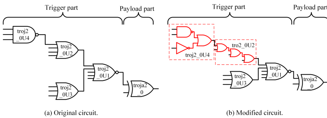
Fig. 6. Gate modification attack on S13207-T002.
