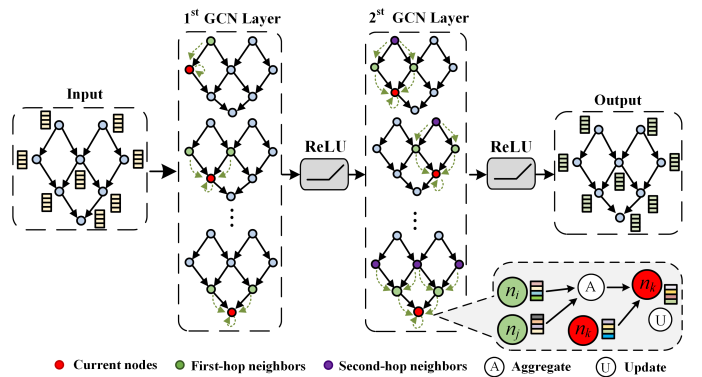
Fig. 3. GCN aggregating neighbor node features.
