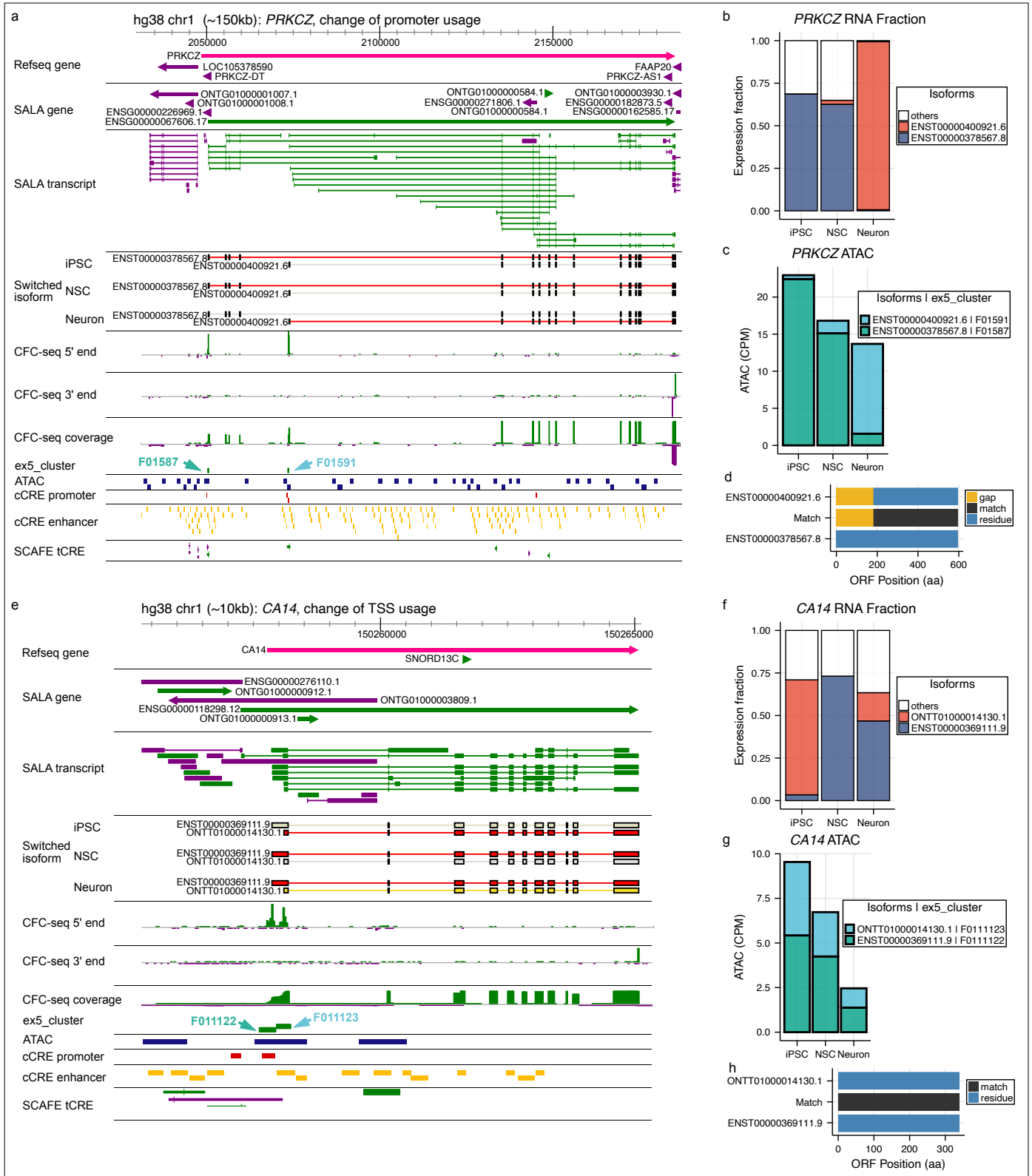
Supplementary Figure 3 | Example genes with significant isoform switching due to switched promoter and TSS usage.
