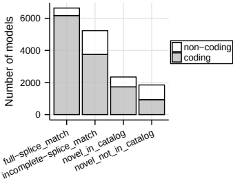
Class of novel isoforms from coding genes
