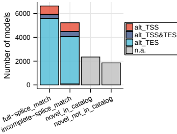
Class of novel isoforms from coding genes
