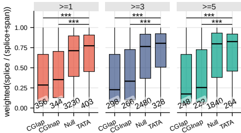
Splicing efficiency per e_ncRNA ex5_cluster
