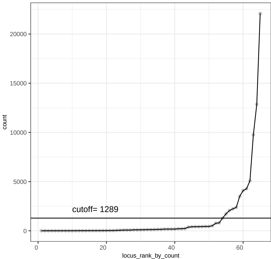
optimize_hyperactive_count
