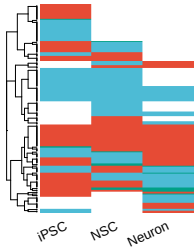
Transcribed enhancer 20,951
