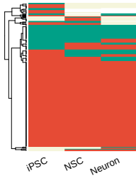
Transcribed promoter 22,341
