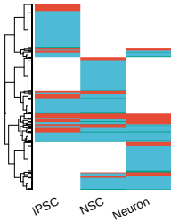
Non-transcribed enhancer 339,753
