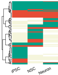
Non-transcribed promoter 12,094
