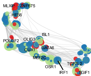
Indirect edges only (TF → enhancer → promoter(TF))
