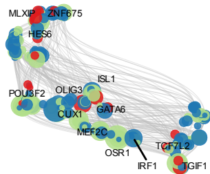
Direct edges only (TF → promoter(TF))
