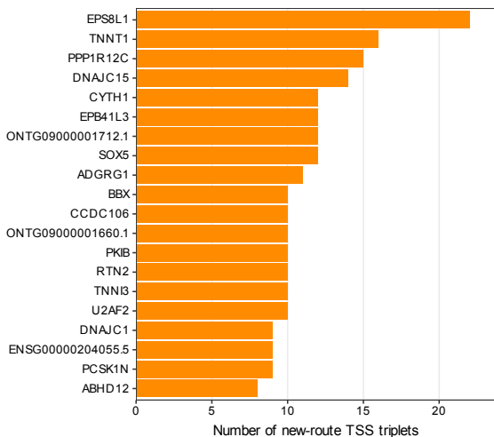
Top 20 target genes gaining the most new TSS routes
