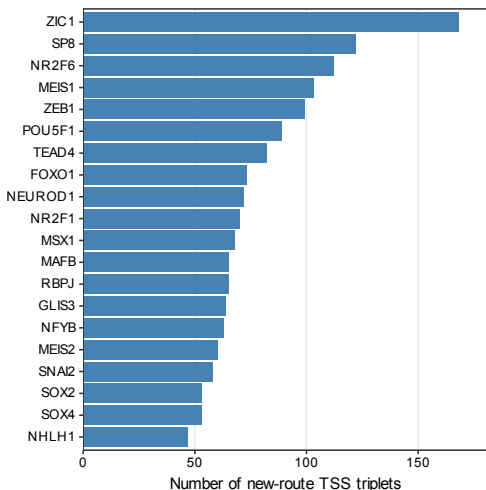
Top 20 target genes gaining the most new TSS routes
