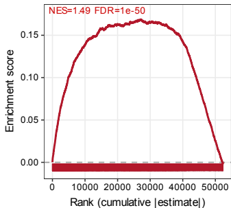
Expressed enhancers
