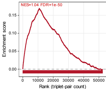
Expressed enhancers
