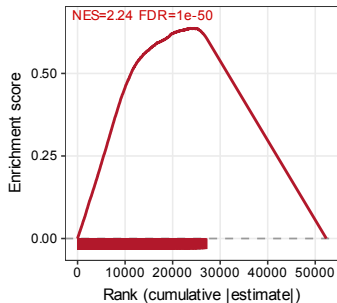
Mediating enhancers
