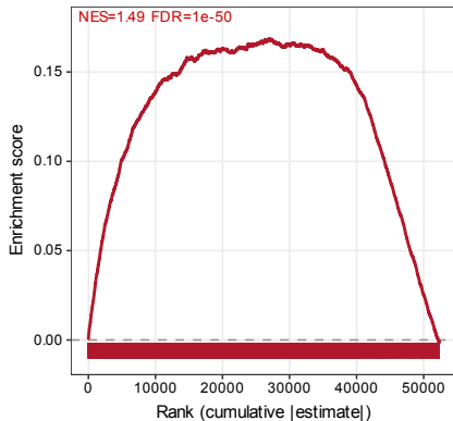
Expressed enhancers
