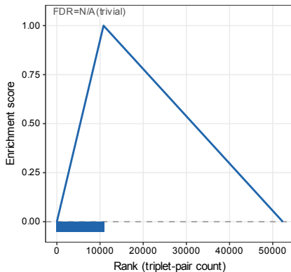
Mediating enhancers
