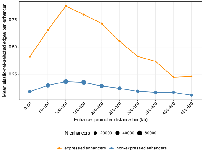
Elastic-net-selected edges per enhancer by distance bin (without-TSS network) expressed vs non-expressed (equal-footing control)
