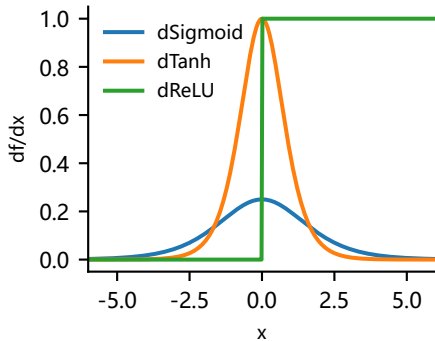
Activation derivatives
