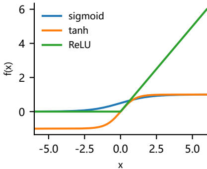
Activation
