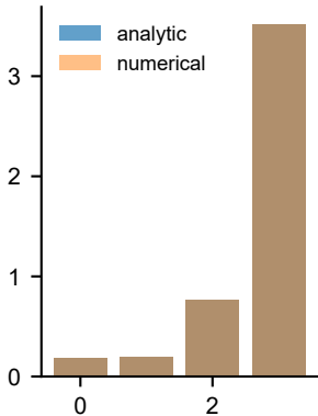
dW2 \frac{1}{2} \frac{d^2 W}{dx^2} vs \frac{d^2 W}{dx^2}
