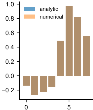
dW1 \frac{1}{2} \frac{d^2 W}{dx^2} vs \frac{d^2 W}{dx^2}
