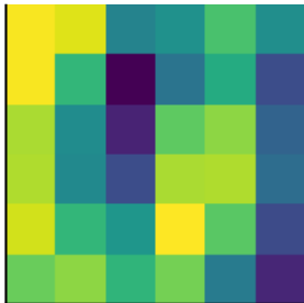
卷积核: emboss
