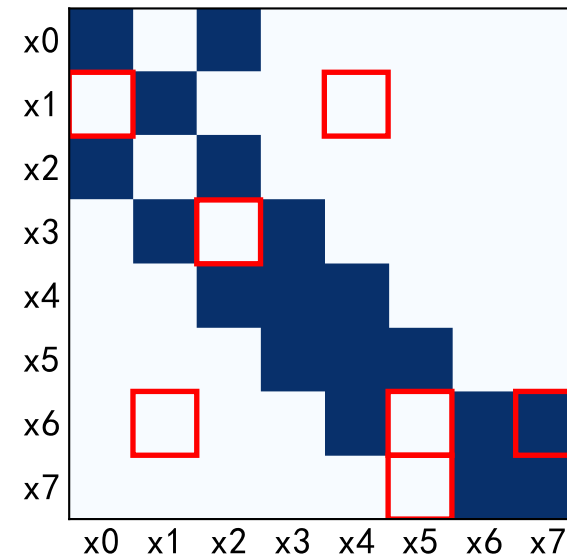
TS-GC (SNR=5dB)
