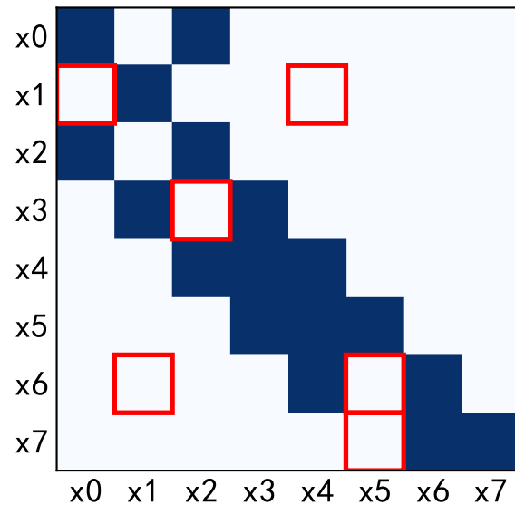
TS-GC (SNR=20dB)
