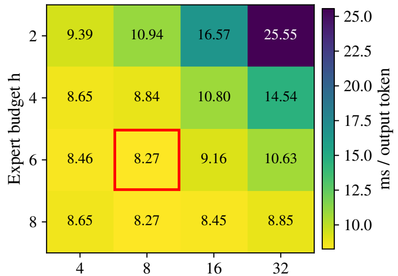
(b) Qwen3.6
