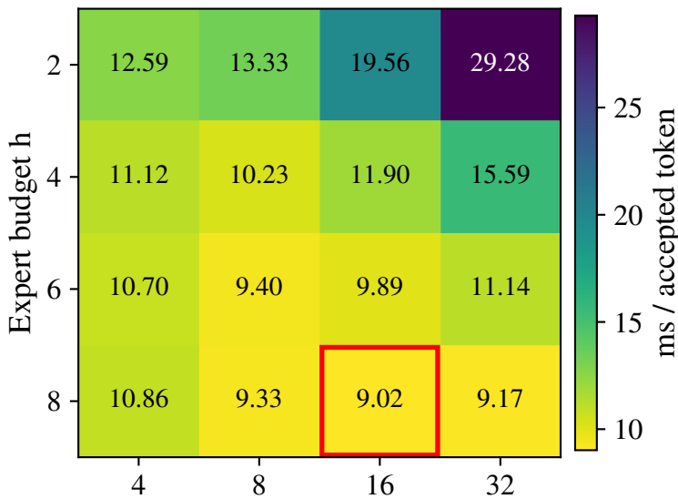
(a) Qwen3.6
