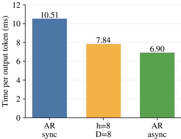
(a) Qwen3.6
