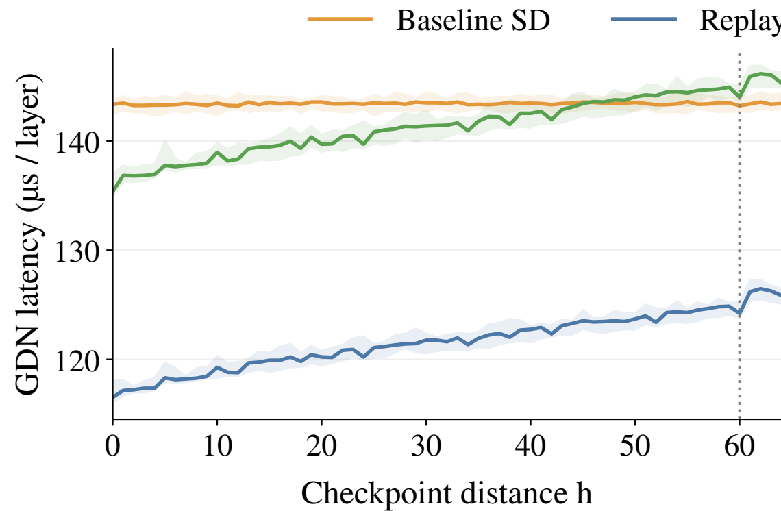
(a) Draft = 4
