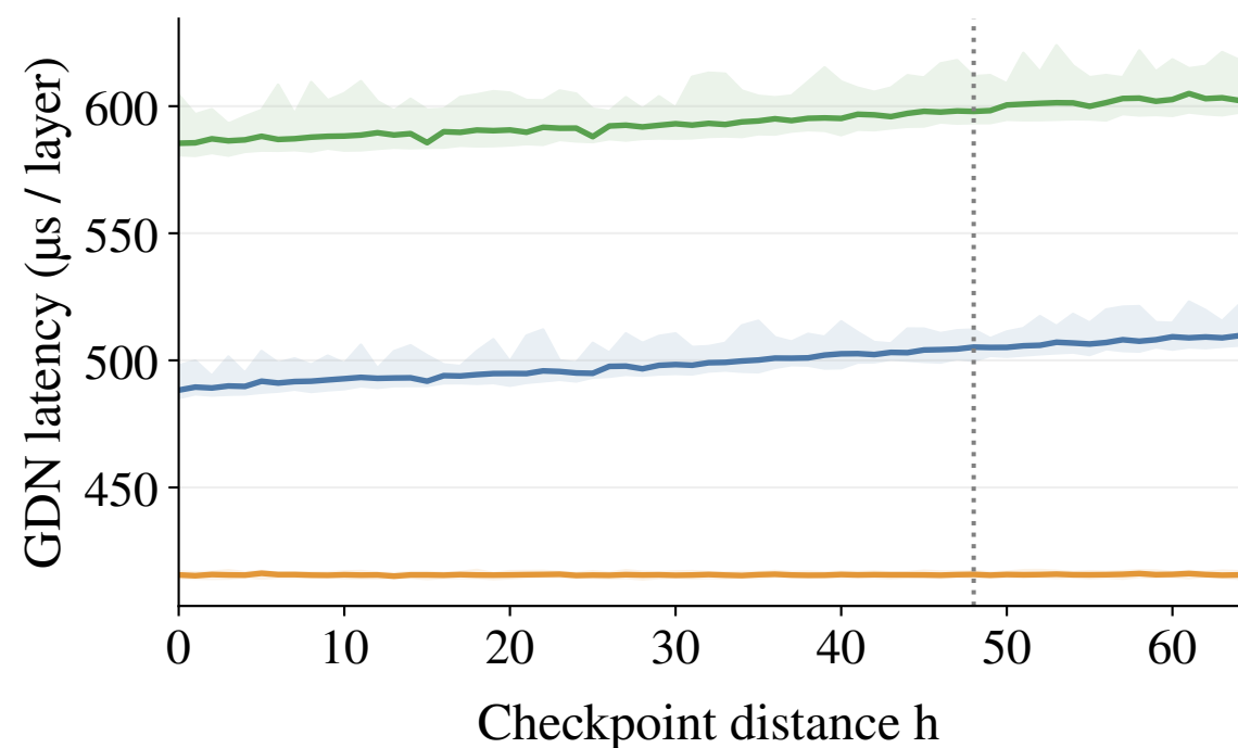
(c) Draft = 16
