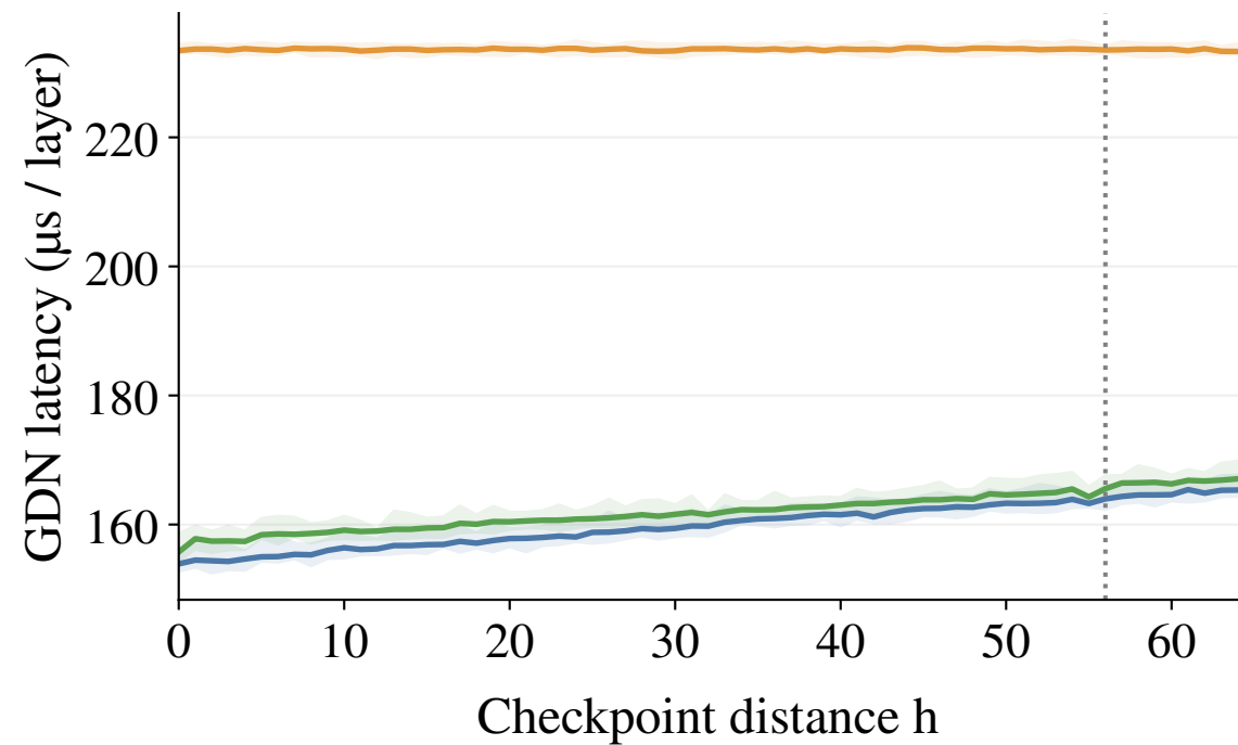
(b) Draft = 8
