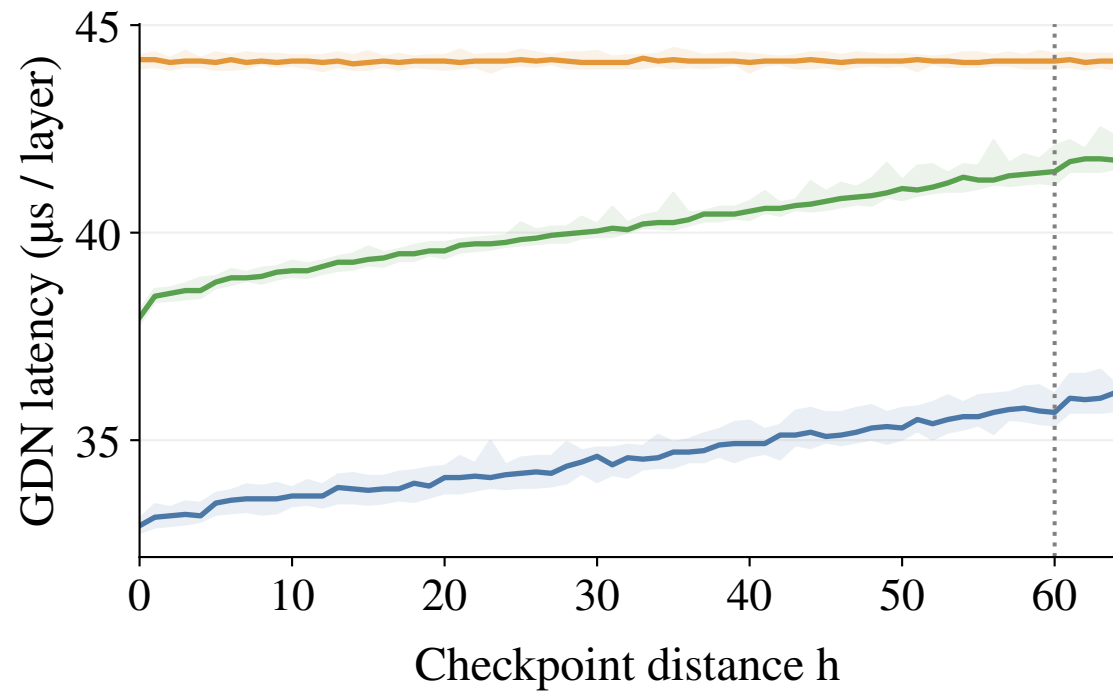
(a) Draft = 4
