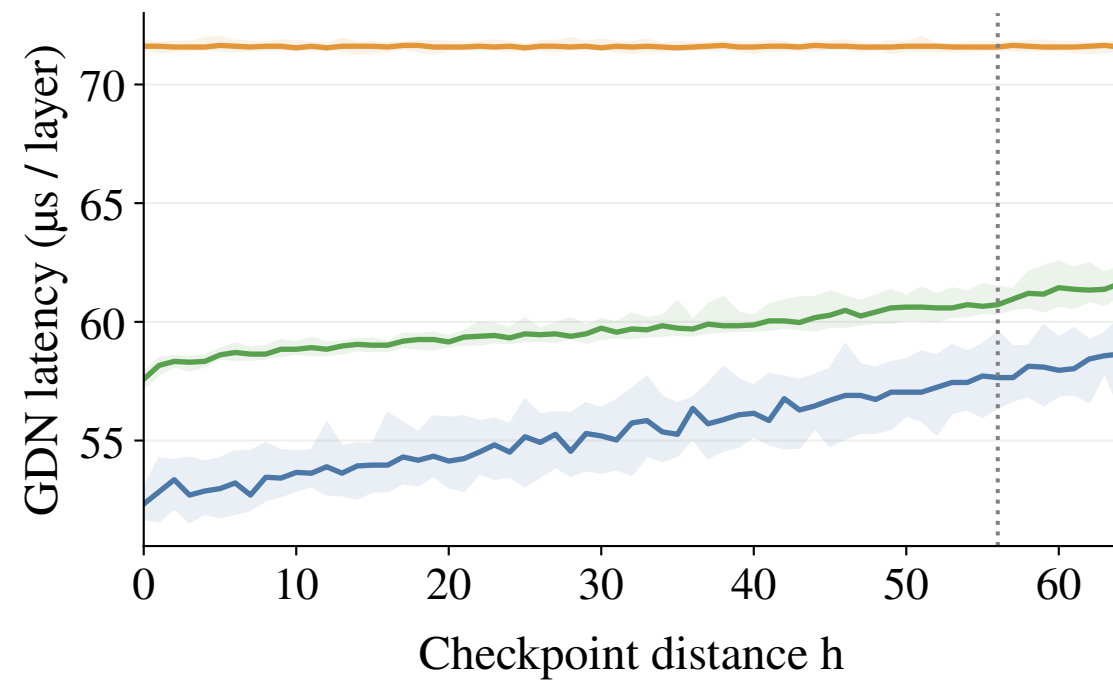
(b) Draft = 8
