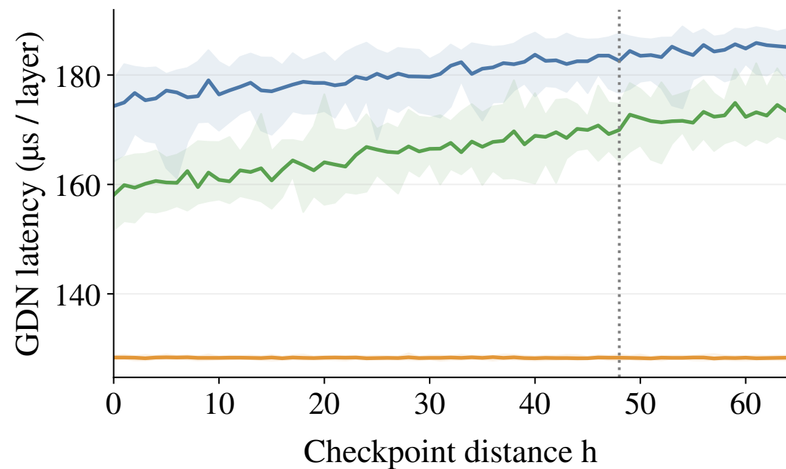
(c) Draft = 16
