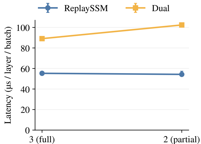
Accepted drafts (b) bs=8, two-window pair
