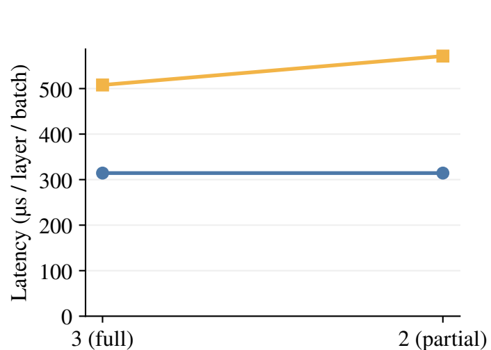
Accepted drafts (c) bs=64, two-window pair
