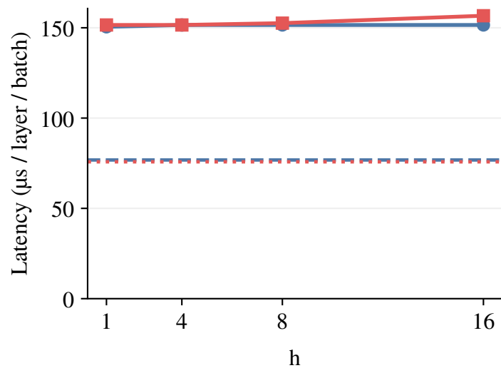
(c) bs=64
