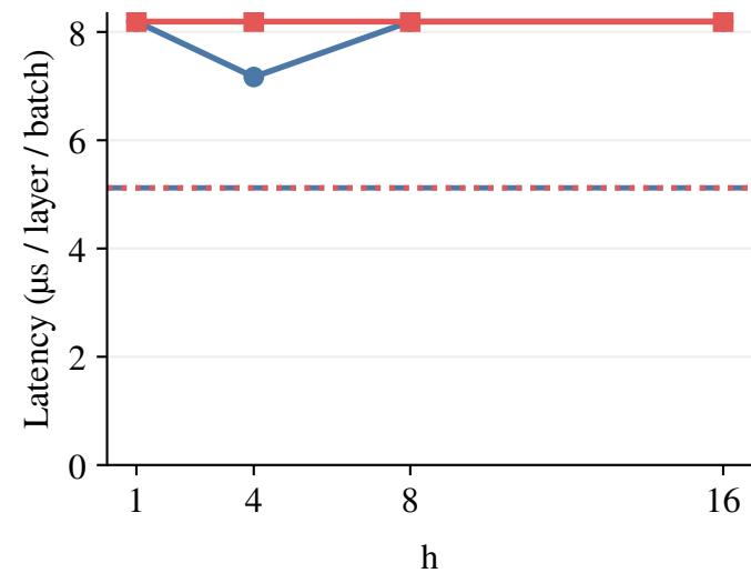
(a) bs=1
