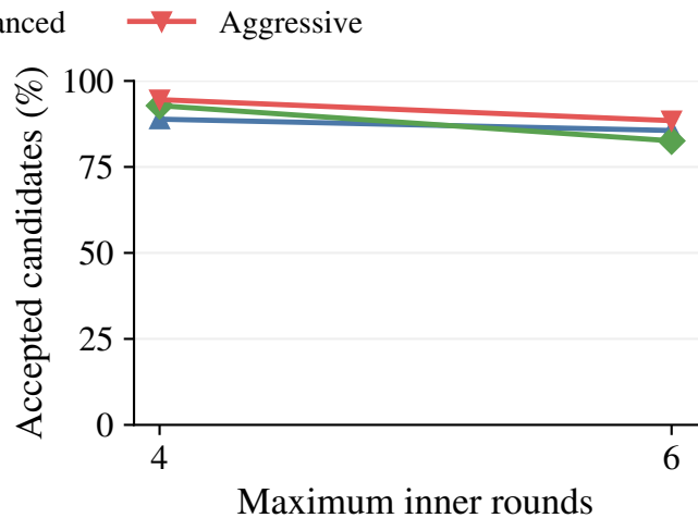
(b) Acceptance
