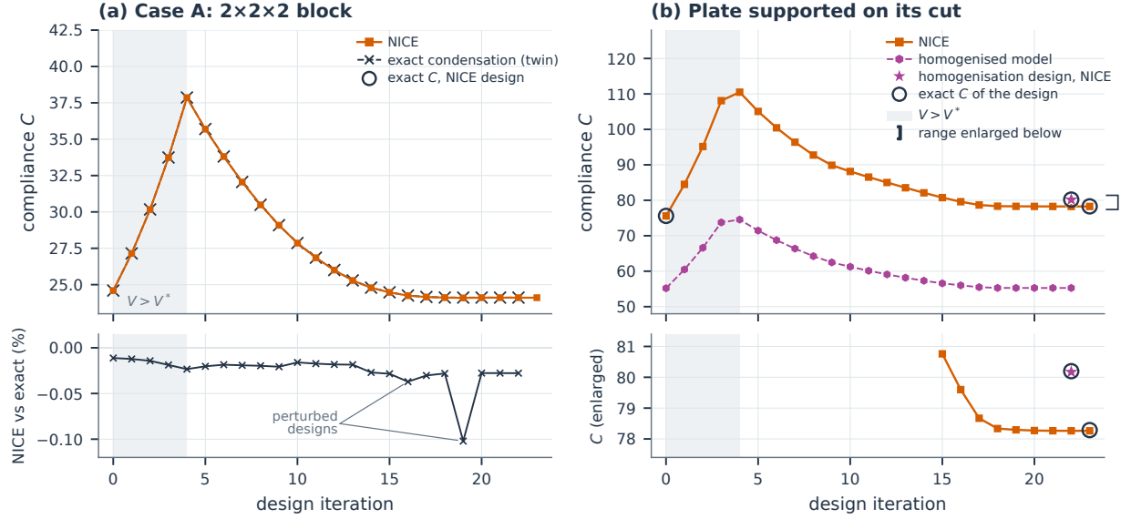
Figure 12: Thickness optimisation with NICE. (a) Case A: compliance histories of the NICE optimisation and of the twin optimisation with exact condensation, with the exact compliance of the NICE designs at iterations 0, 12 and 23 (open circles); the compliance first rises while the volume is reduced from 1.25V^* to V^* (shading, iterations 0–3). Lower strip: NICE compliance relative to the twin run at the same design iteration (line; the designs of the two runs coincide at iterations 0–4 and differ afterwards) and to the exact compliance of the same design (circles: -0.011\% , -0.018\% , -0.028\% ); at iterations 16 and 19 (labelled 'perturbed designs') the geometry-generation fallback had perturbed the NICE design (Supplementary Note S9.4, Table ST24a). (b) Plate supported on its cut: NICE compliance from the uniform start, compliance of the homogenised macroscale model along its own optimisation (dashed), the homogenisation design analysed with NICE on the cut geometry (star, at the last macroscale iteration) and the exact compliance of the uniform start, the final NICE design and the homogenisation design (open circles). Shading: design iterations with V > V^* . Lower strip: the range marked by the bracket, enlarged, from iteration 15.
