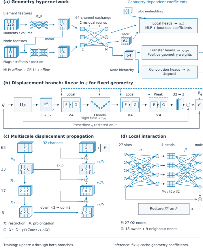
Figure 3: Geometry-conditioned neural displacement architecture. (a) Element and node encoders produce 64-channel geometry embeddings, followed by two rounds of residual exchange; coefficient heads condition the local interactions, grid transfers and convolutions. (b) The displacement branch propagates the nonrigid retained input through four local interaction pairs, the multilevel block, four further local pairs and four pairs on weakly supported stencils; linear maps connect the three displacement components to 32 latent channels, and deterministic bypasses reconstruct rigid motion and restore the retained values. (c) Restriction and prolongation connect grids with 65, 33, 17 and 9 background positions per axis; each coarse level has two residual convolutions on each pass. (d) A local interaction uses geometry-weighted gathering, four channel-mixing heads and scattering, followed by residual addition and retained-value restoration. E and G denote element and ghost-face interactions. Blue dashed arrows carry geometry-dependent coefficients; solid arrows carry features or displacement states. For fixed geometry, the complete displacement path is linear.
